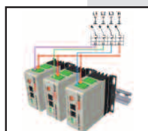
Collegamento 3F. 3 Phase wiring diagram.
